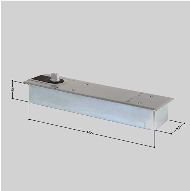
Floor spring GEZE Stop TS550NV
